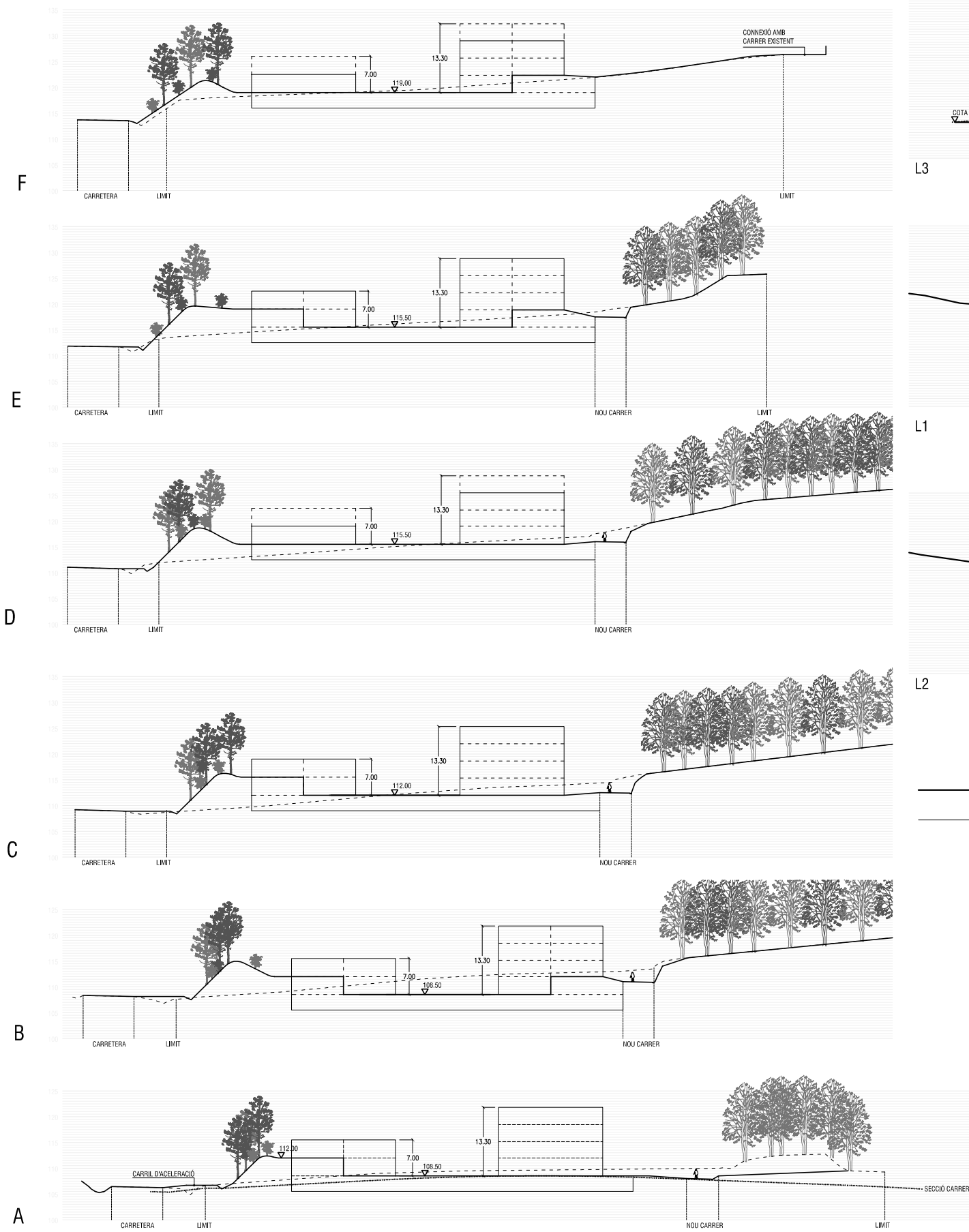
SECCIONS TRANSVERSALS INDICATIVES E 1:1000
